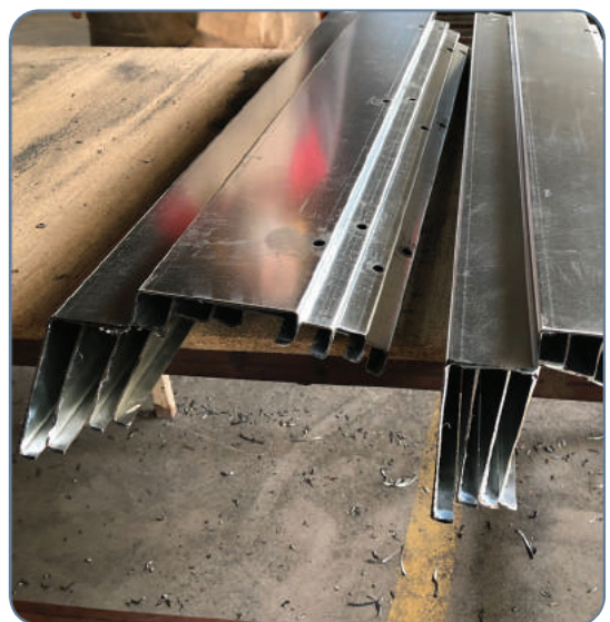
Frame Detail
